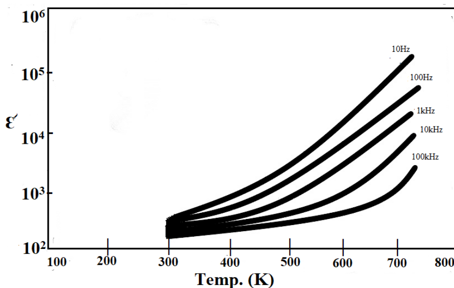
Figure 5. Increase in dielectric constant with temperature
