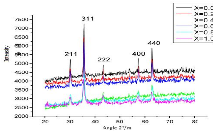
Figure 1. XRD patterns of \text{Cu}_{0.5}\text{Co}_{x/2}\text{Zn}_{0.5}\text{Fe}_{2-x/2}\text{O}_4
